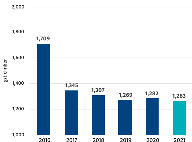
SPECIFIC NO x EMISSIONS
